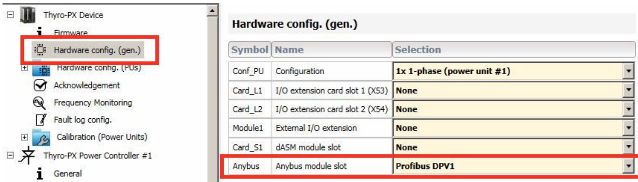
Figure 2. Menu tree
